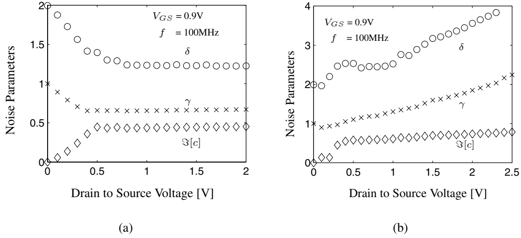
FIGURE 1. Drain bias evolution of three noise parameters ( \gamma , \delta , and the imaginary part of c ) comparing long channel characteristics with short channel. (a) 5\ \mu\text{m} nMOSFET. (b) 0.25\ \mu\text{m} nMOSFET.
