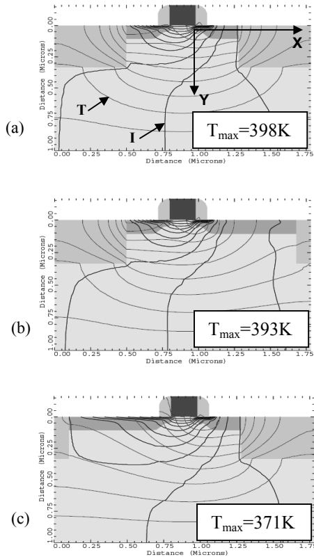
FIGURE 17. The current flowline and temperature distribution contours at the drain current of 1\text{mA}/\mu\text{m} for the three different structures are shown. (a) GSCS= 0.1\mu\text{m} and GDCS= 0.1\mu\text{m} , (b) GSCS= 0.1\mu\text{m} and GDCS= 0.5\mu\text{m} , and (c) GSCS= 0.5\mu\text{m} and GDCS= 0.1\mu\text{m}
