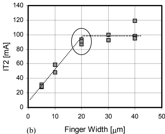
FIGURE 8. Total failure threshold current ( I_{T2} ) with the finger width for (a) 1.5V NMOS transistors and (b) 3.3V NMOS transistors where GDCS/GSCS=0.1 µm. The total failure current can be scaled with finger width within only a limited finger width ( W \leq 20 \mu\text{m} ) for the 3.3V devices. The overall data show the strong current localization for the salicided devices under ESD stress.
