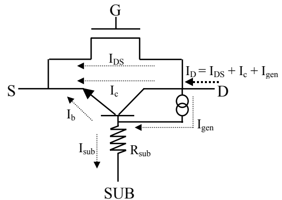
FIGURE 10. Equivalent circuit of the NMOS including the parasitic lateral NPN bipolar transistor when the LNPN is on.
