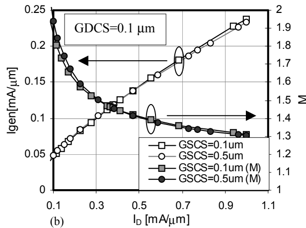
FIGURE 12. The avalanche-generation current ( I_{gen} ) and multiplication factor ( M ) for the variation of (a) the GDCS and (b) GSCS.
