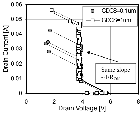
FIGURE 7. High current TLP curves for the 1.5V NMOS transistor with two different GDCS of 0.1µm and 1µm where GSCS is 0.1 µm. The slope of high current regions is almost identical, but the failure threshold current ( I_{T2} ) is nearly doubled with the increased GDCS.
