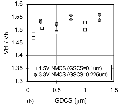
FIGURE 13. To track the current gain of a lateral NPN transistor, the triggering voltage ( V_{t1} ) and holding voltage ( V_h ) are measured for the 1.5V and 3.3V NMOS transistors. The data clearly show that the current gain is reduced by increase in GSCS (a), while remains nearly constant with GDCS (b).
