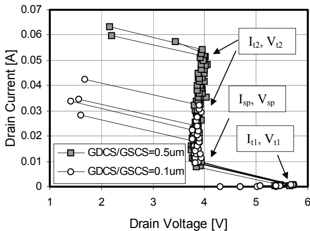
FIGURE 3. High current TLP curves for the 1.5V NMOS transistor with two different GDCS/GSCS (0.1 \mu\text{m} and 0.5 \mu\text{m} ), which clearly show the impact of the gate-to-contact spacings on I_{t2} despite the silicided diffusion.
