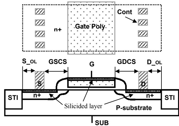
FIGURE 1. The schematic of a salicided NMOS transistor indicating the gate to source/drain contact spacing (GSCS/GDSCS) and the n^+ overlap of the source/drain contact ( S_{OL}/D_{OL} ). For the 1.5V NMOS, the S/D contact opening ( S/D ) = 0.15 \mu\text{m} and S_{OL} = D_{OL} = 0.1\mu\text{m} . For the 3.3V NMOS, the S/D contact opening ( S/D ) = 0.15 \mu\text{m} and S_{OL} = D_{OL} = 0.125\mu\text{m} . In the test structures, the S/D contact opening and n^+ overlap of S/D contact ( S_{OL}/D_{OL} ) remain unchanged despite the variations of GSCS/GDSCS.
