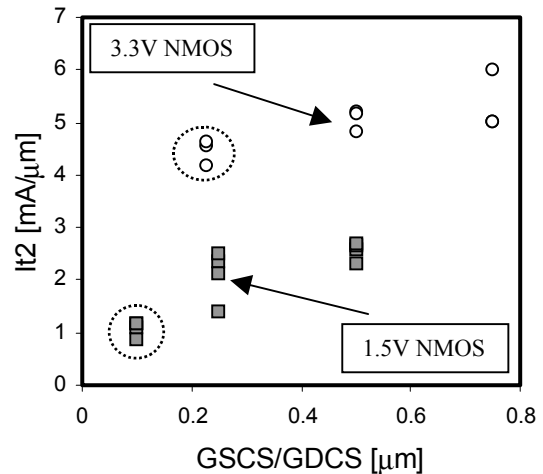
FIGURE 4. The second breakdown triggering current ( I_{t2} ) with the gate-to-source/drain contact spacing for two different silicided NMOS transistors. The two dashed circles indicate I_{t2} for each device with minimum contact spacing (0.1 \mu\text{m} and 0.225 \mu\text{m} for the 1.5V NMOS and 3.3V NMOS, respectively). Squares represent the 1.5V NMOS transistors ( W/L_{poly} = 20/0.175 \mu\text{m} ), and circles represent the 3.3V NMOS transistors ( W/L_{poly} = 20/0.5 \mu\text{m} ).
